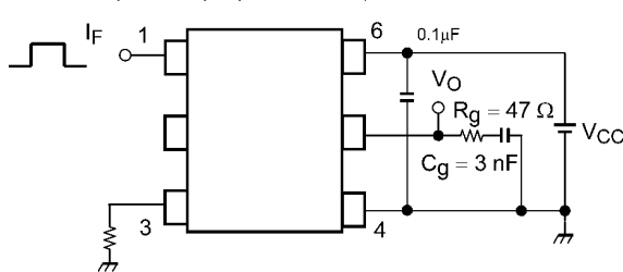
Fig. 13.1.7 Switching Time Test Circuit and Waveform
