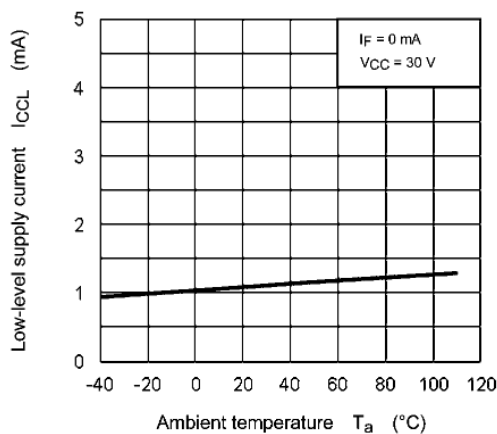
Fig. 13.2.5 I_{CCL} - T_a
