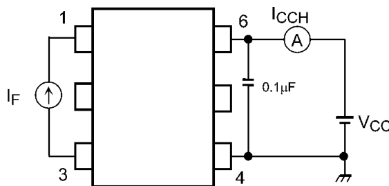
Fig. 13.1.5 I CCH Test Circuit
