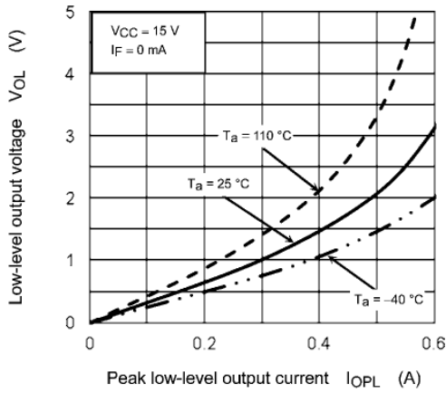
Fig. 13.2.9 V_{OL} - I_{OPL}
