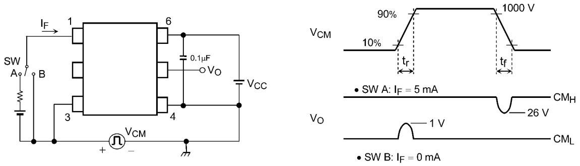
Fig. 13.1.8 Common-Mode Transient Immunity Test Circuit and Waveform
