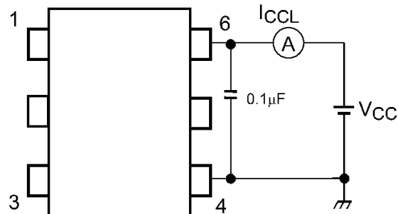
Fig. 13.1.6 I CCL Test Circuit
