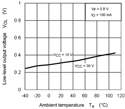
Fig. 13.2.7 V_{OL} - T_a
